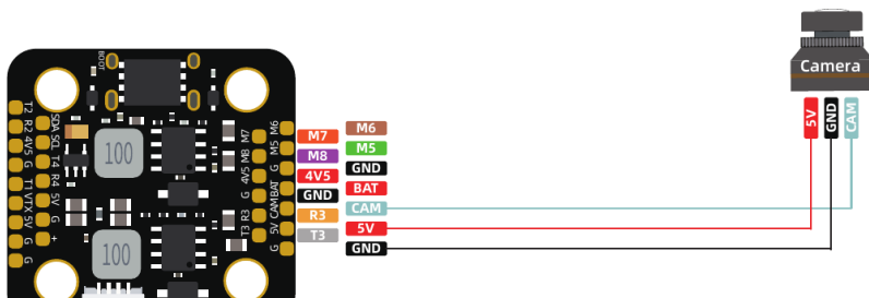
Connecting an FPV camera
