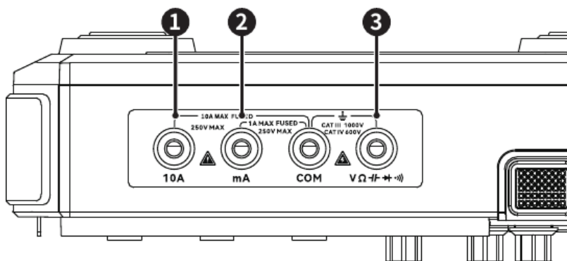
Test lead sockets
