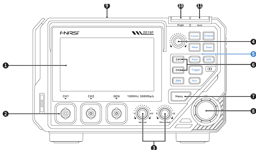
Front panel of the instrument
