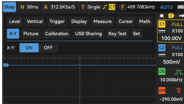
XY mode setup
